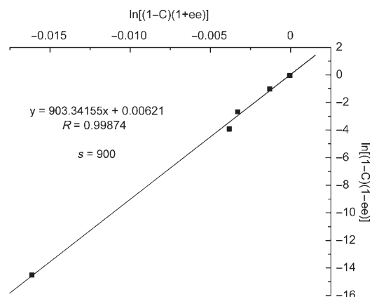
Figure 1. Determination of the selectivity factor by linear regression based on recovered ( R )- 2 ( C = \text{conv}/100 , ee = ee/100 , s = 900 ).
